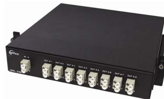
Optical Passive Splitter, OPS-xyz
